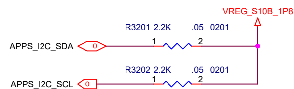
APPS Processor I2C
