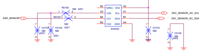
SAR sensor
