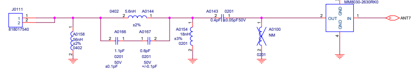
ANT7_GPSL1_WIFI_2.4G
