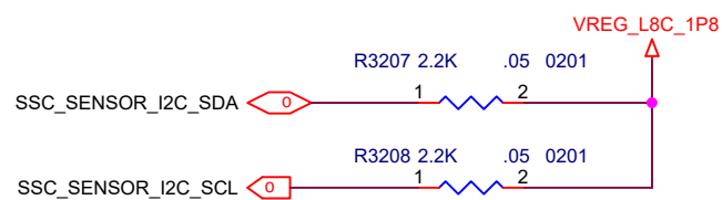
SENSOR I2C4
