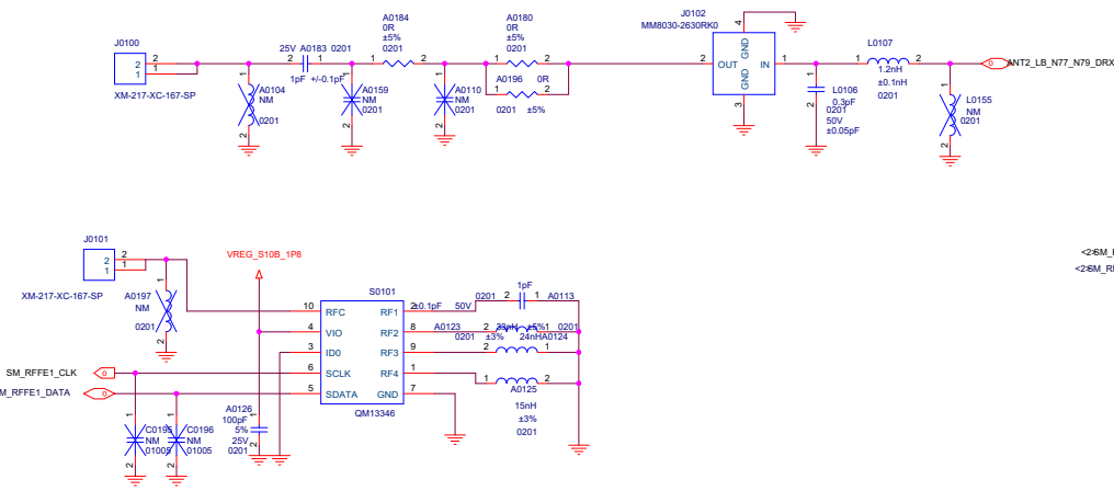
ANT2_LB_N77_N79_DRX
