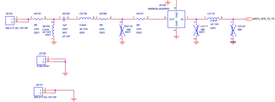
ANT5_N78_79_TX1
