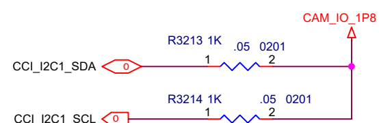
Camera I2C1
