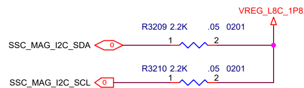
I2C for MAG Sensor
